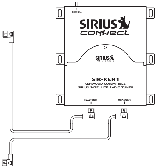
Optional Kenwood SIRIUS-READY Headunit (5L-Bus CD Player or Mobile Multimedia Station)
